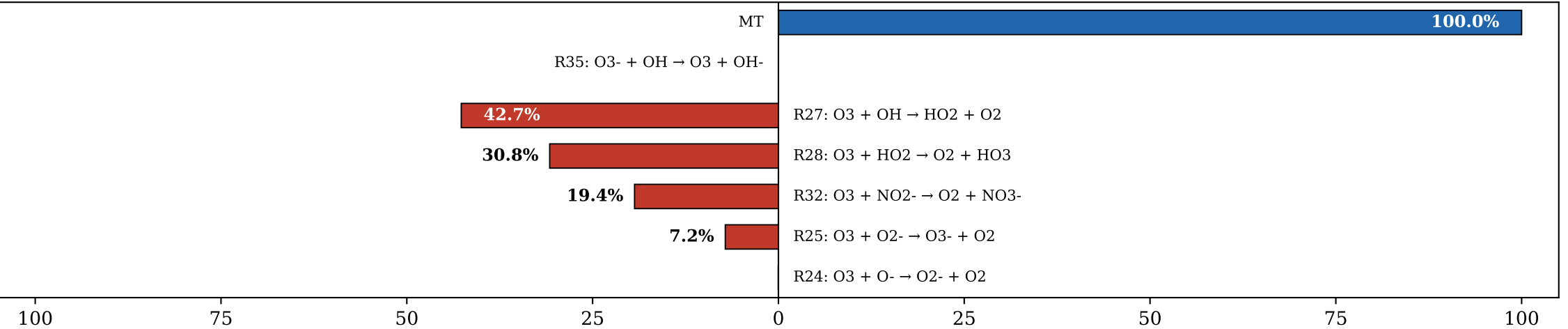
(c) NO 2 - (Σsrc = 1.24e-08 M/s)
